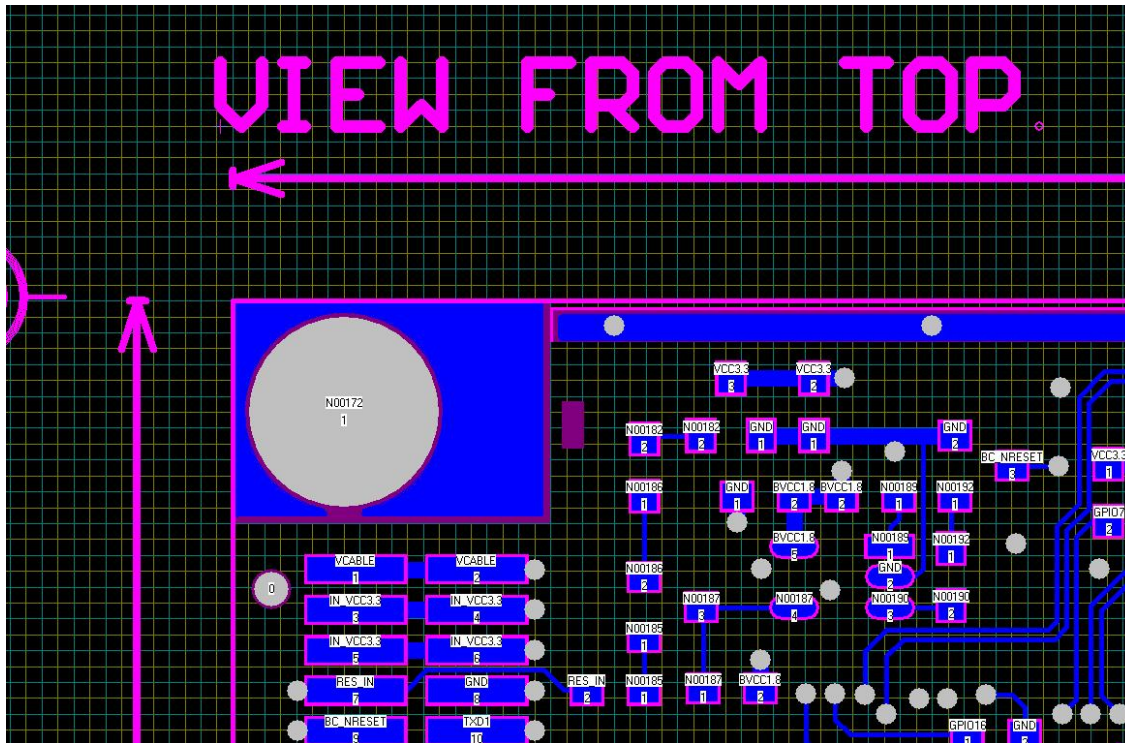
Pin 1 on bottom (Board Upper left corner. View from TOP)
